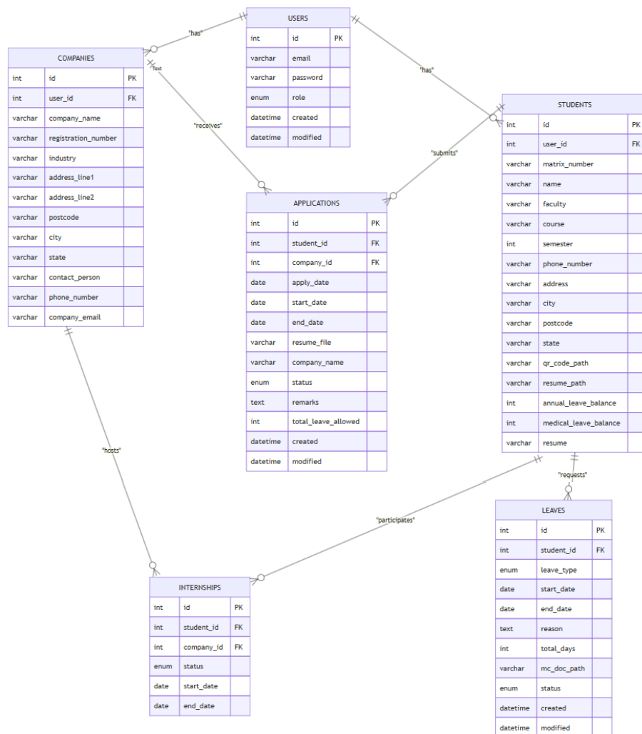
Figure 1: Entity Relationship Diagram of TalentRoute Internship System
